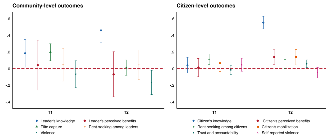
Figure 6: Aggregation: results
